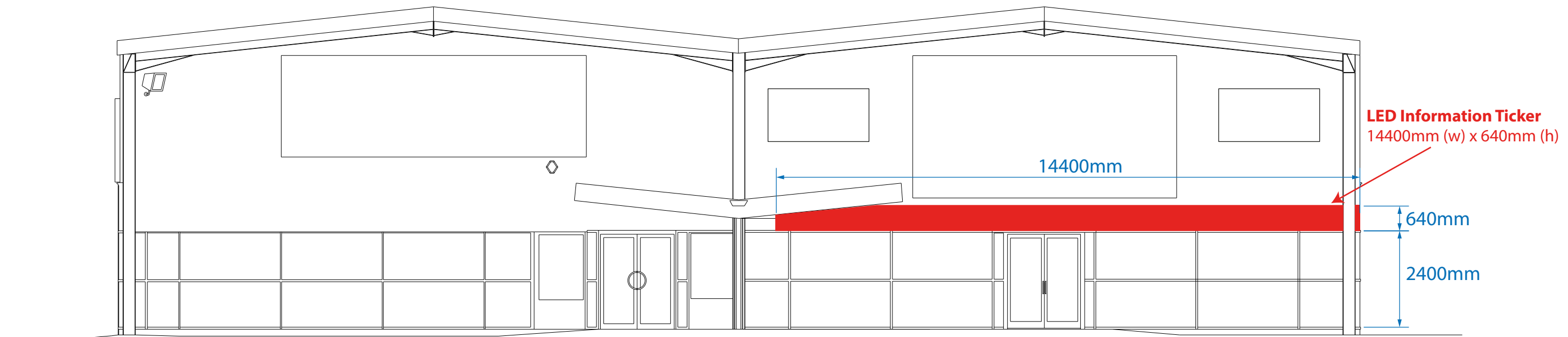
FRONT ELEVATION AS PROPOSED - 1:100 @A3
