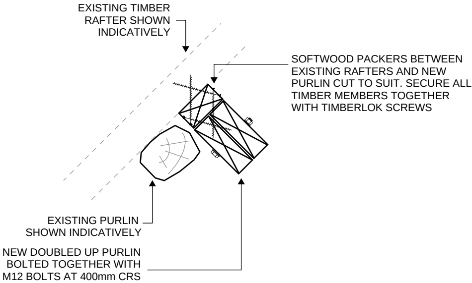
DETAIL 02 NTS 9002 RAFTER CONNECTION TO NEW PURLIN DETAIL
