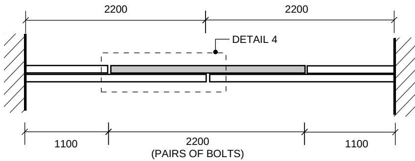
DETAIL 03 NTS 9002 LAYOUT OF NEW SPLICED PURLIN - PLAN
