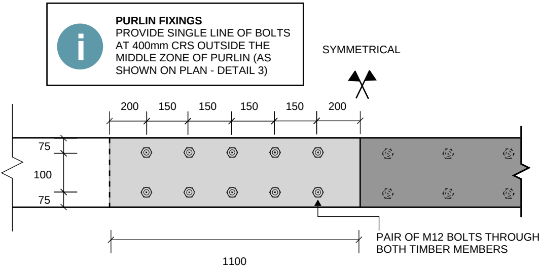
DETAIL 04 NTS 9002 LAYOUT OF NEW SPLICED PURLIN - ELEVATION
