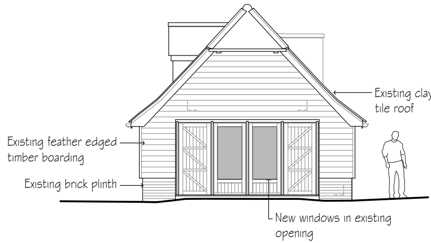
South elevation
