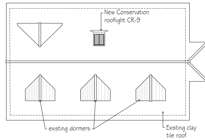
Roof plan
