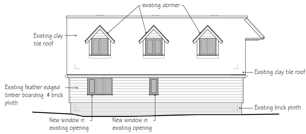
West elevation
