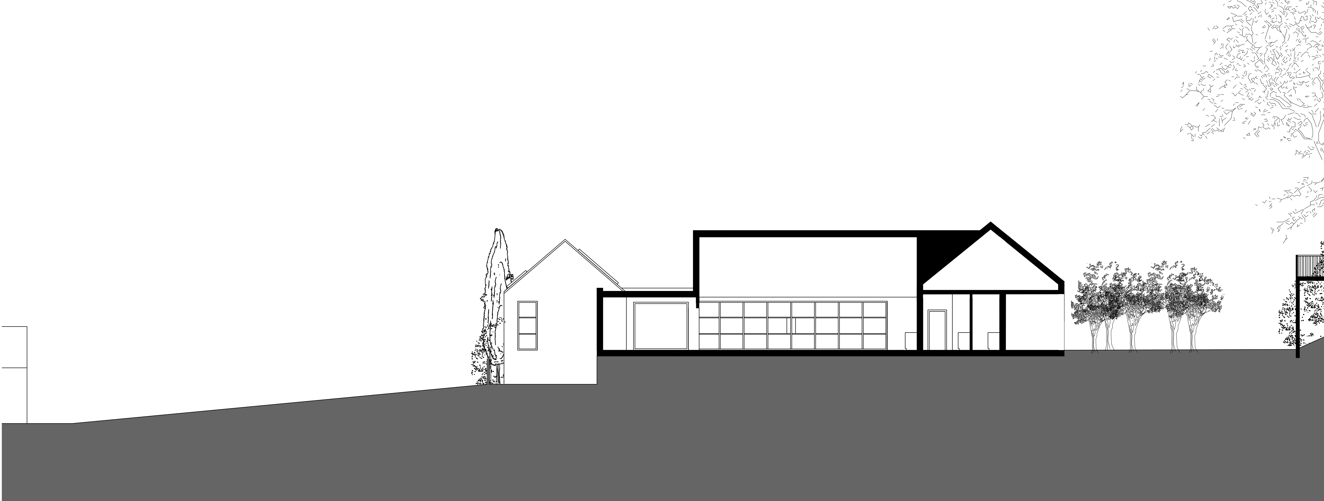
2. Proposed Site Section (B:B)
