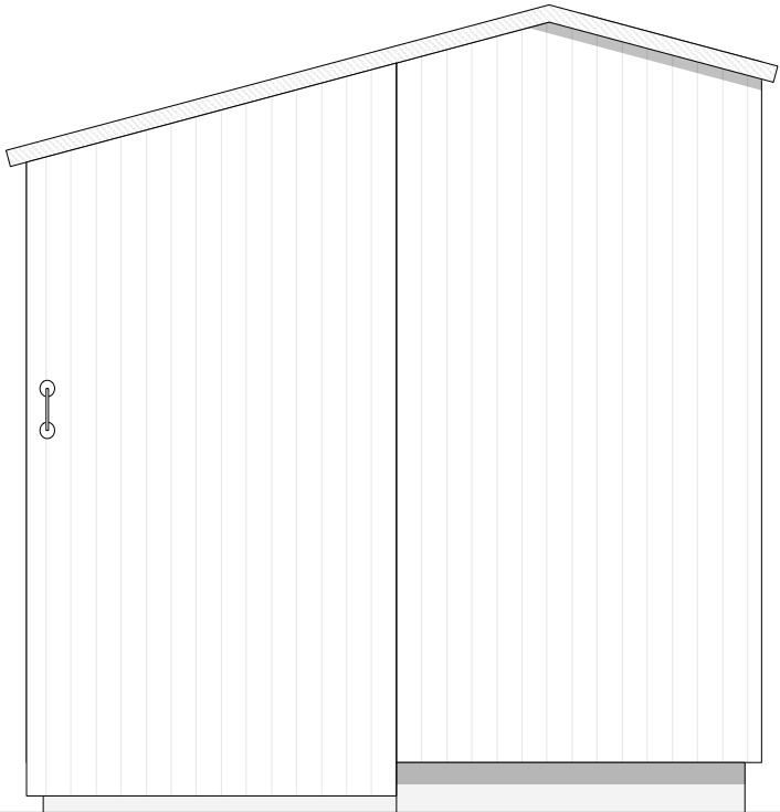
EAST ELEVATION
