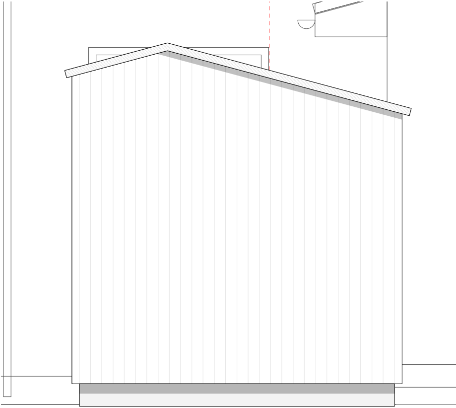
WEST ELEVATION
