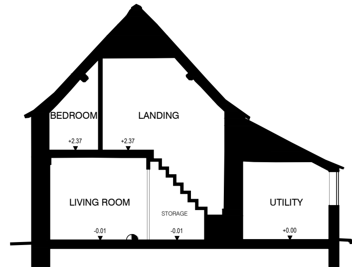
4 EXISTING SECTION AA 4 2 S H U R N H O L D
