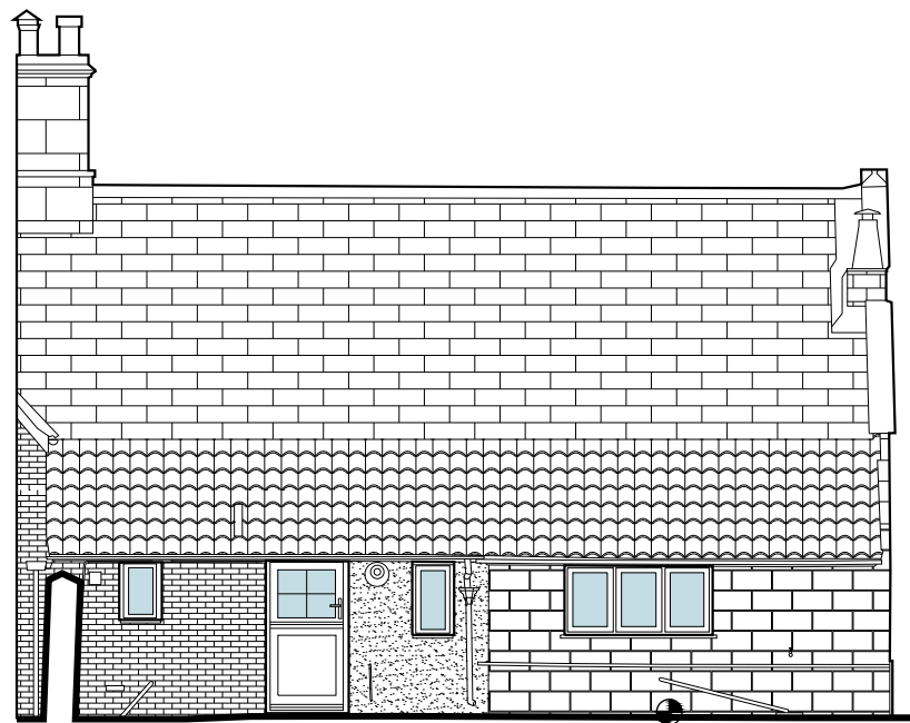
3 EXISTING NORTH EAST ELEVATION 4 2 S H U R N H O L D
