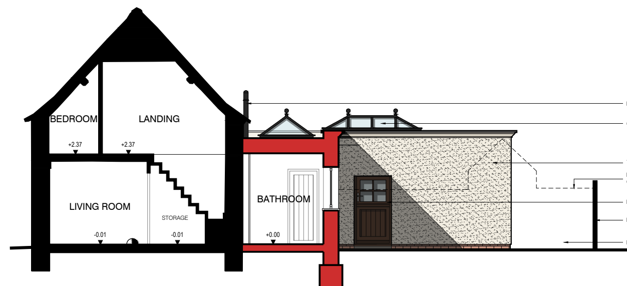
4 PROPOSED SOUTH EAST ELEVATION 4 2 S H U R N H O L D
