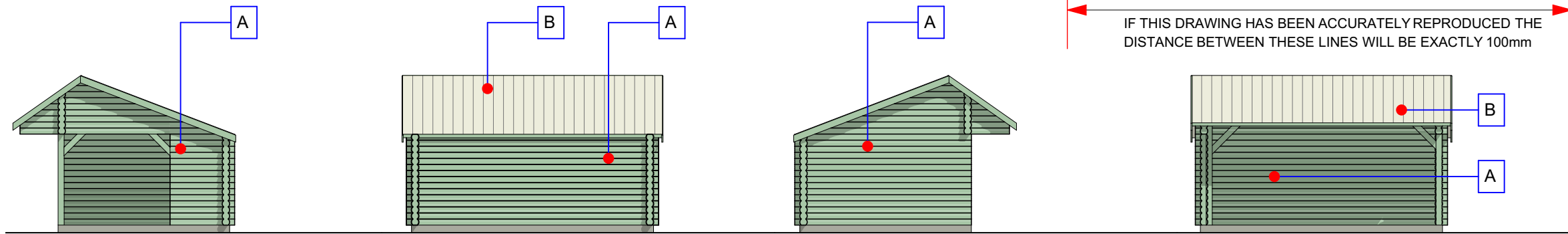
East Elevation - 1:100 North Elevation - 1:100 West Elevation - 1:100 South Elevation - 1:100
