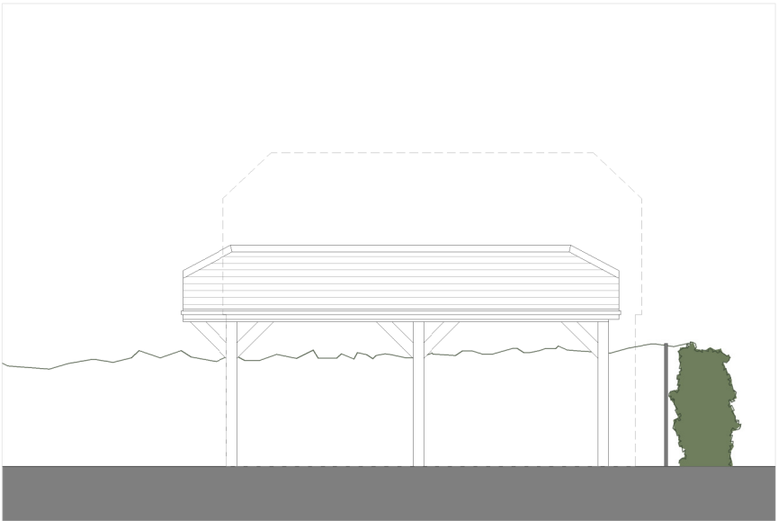
06 - Rear Car Port Elevation
