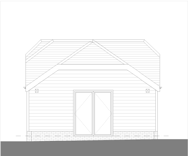
04 - Rear Elevation
