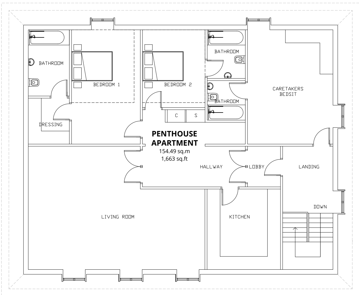
SECOND FLOOR PLAN (LEVEL 04)
