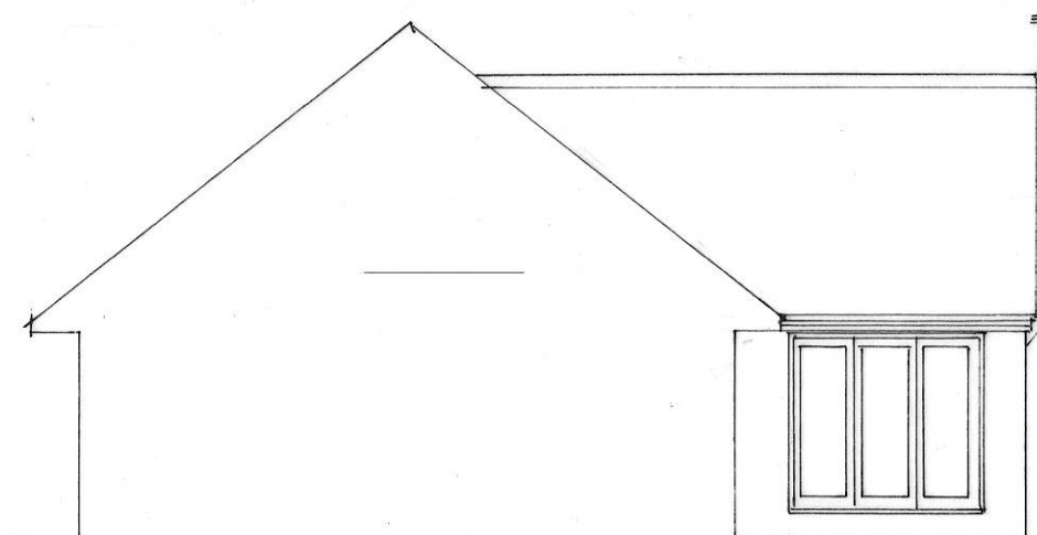
South Elevation
