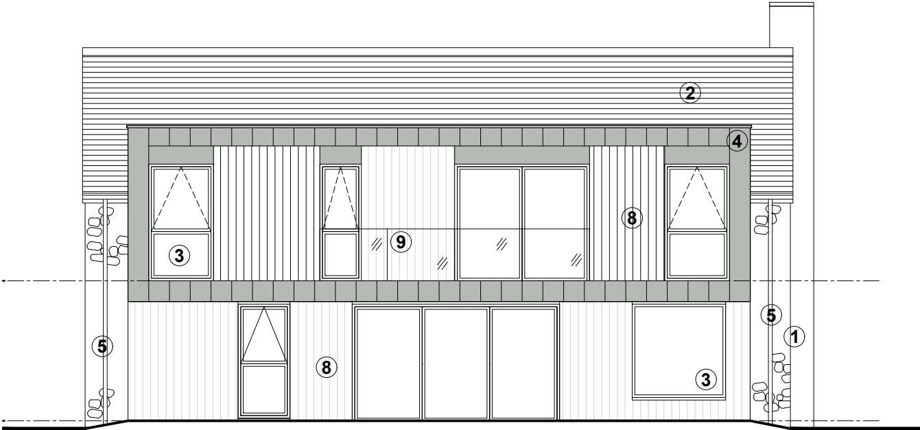
REAR ELEVATION
