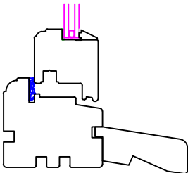
Window Bottom Rail
