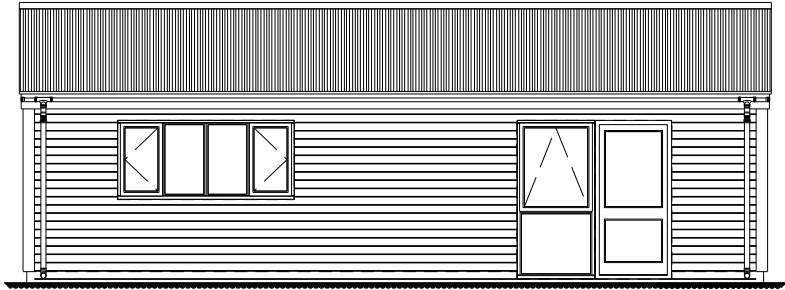
SOUTH ELEVATION
