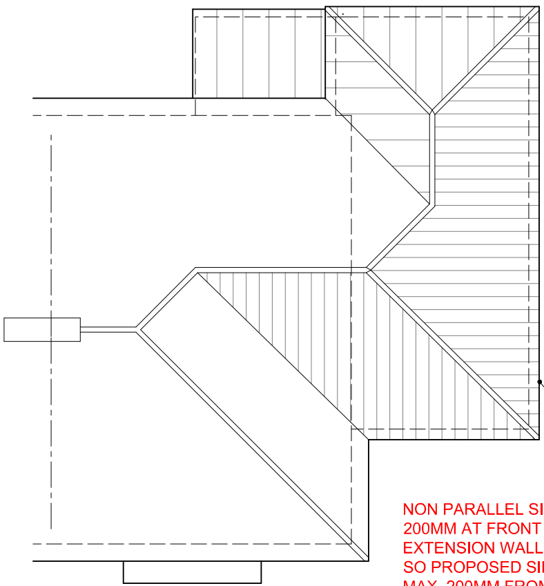
ROOF PLAN
