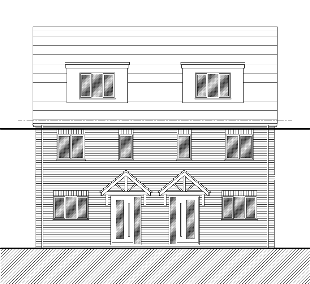
East Elevation
