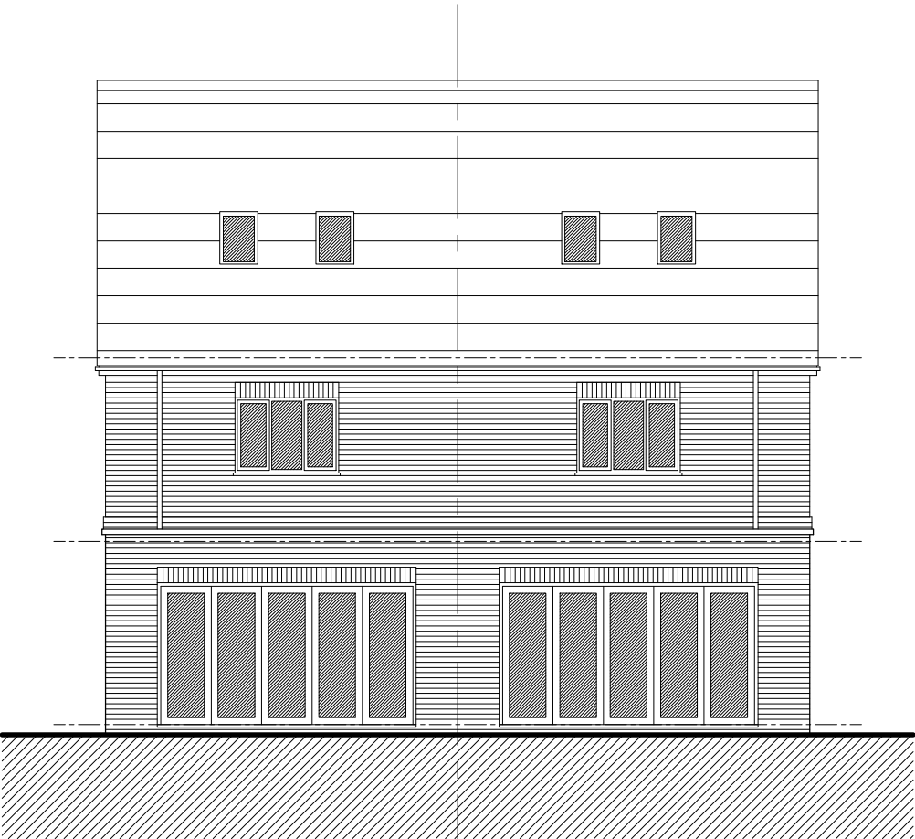
West Elevation
