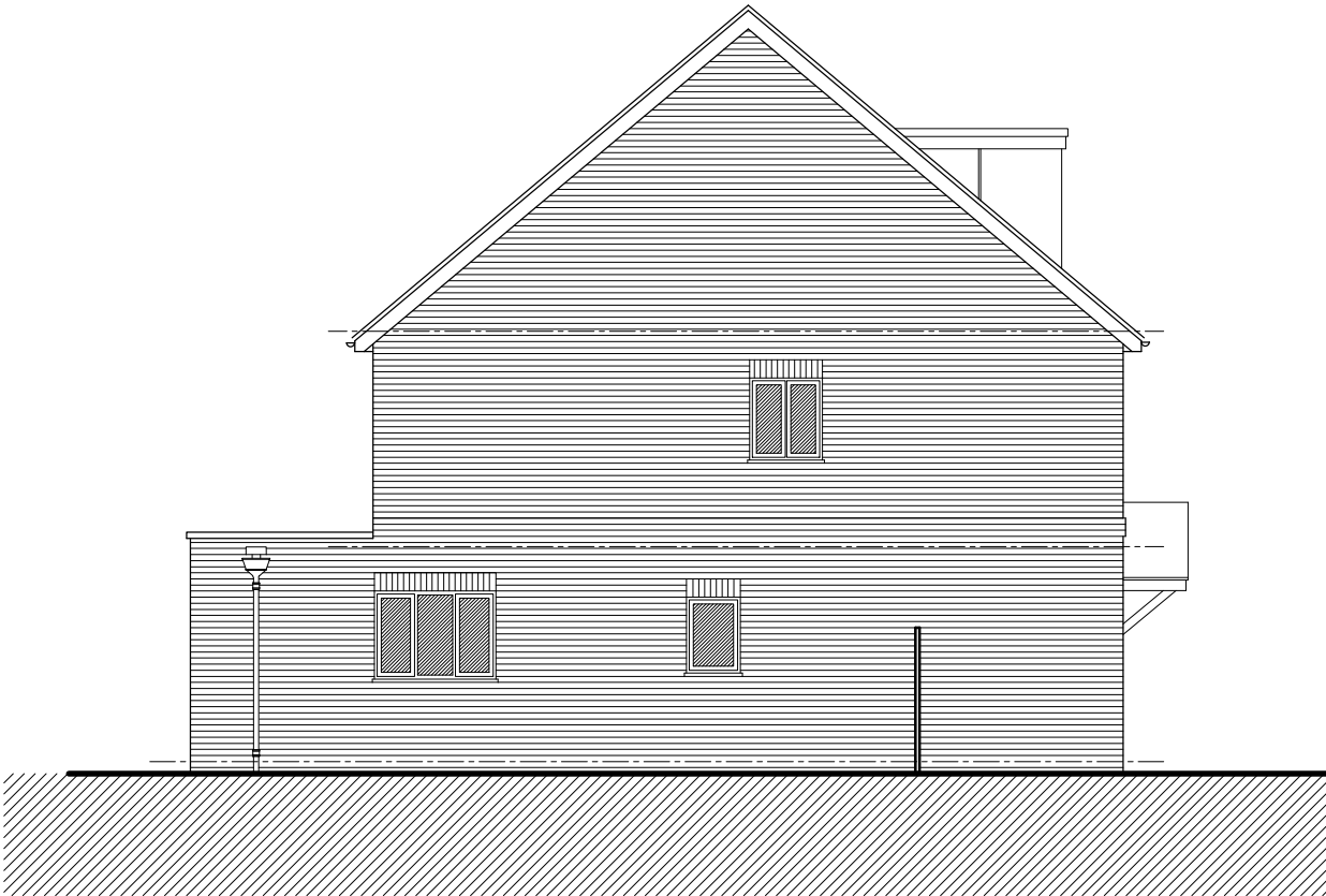
South Elevation
