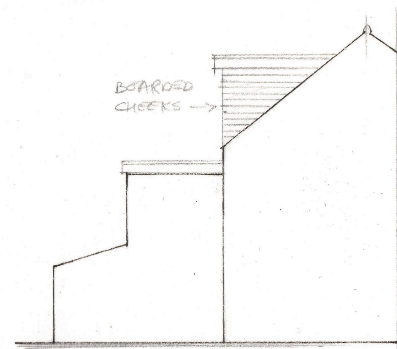
NORTH elevation 1:100
