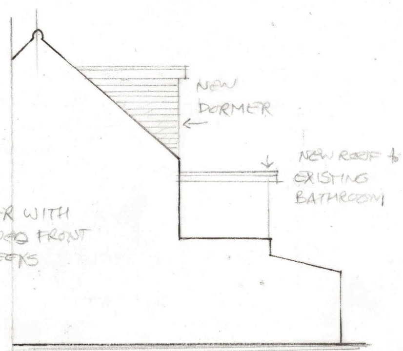
SOUTH elevation 1:100
