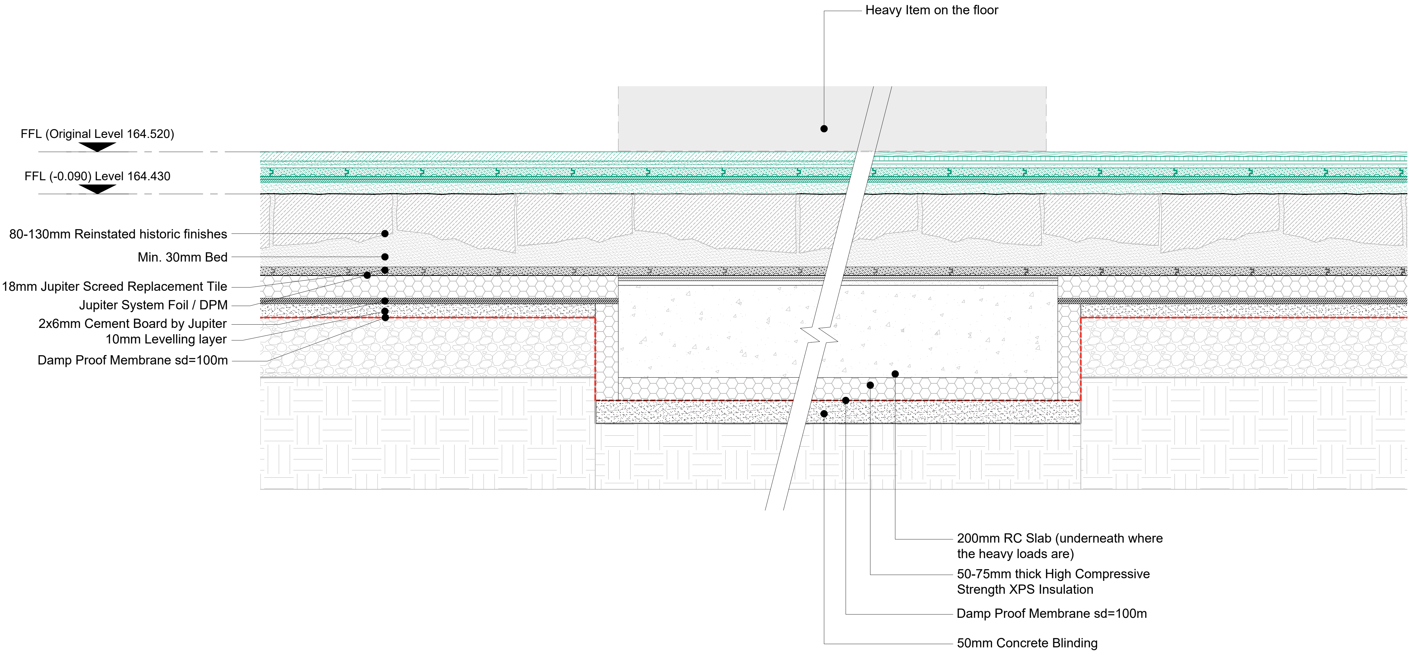
1 Section through the Heavy Loads sitting on the floor 1:5 @ A1 / 1:10 @ A3 - GROUND FLOOR
