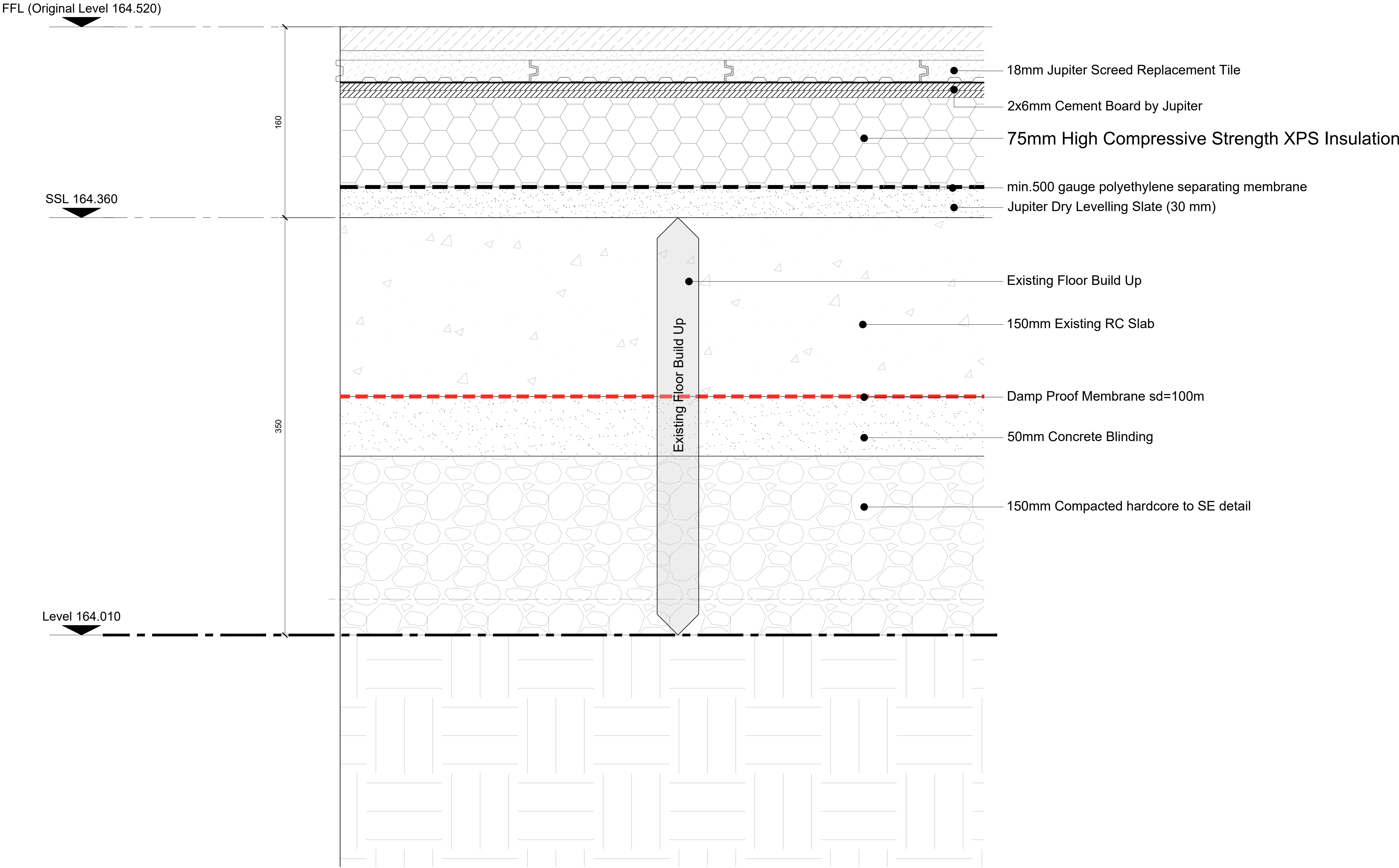
1 Ground Floor Build Ups over existing RC Slab 1:2 @ A1 / 1:4 @ A3 - GROUND FLOOR
