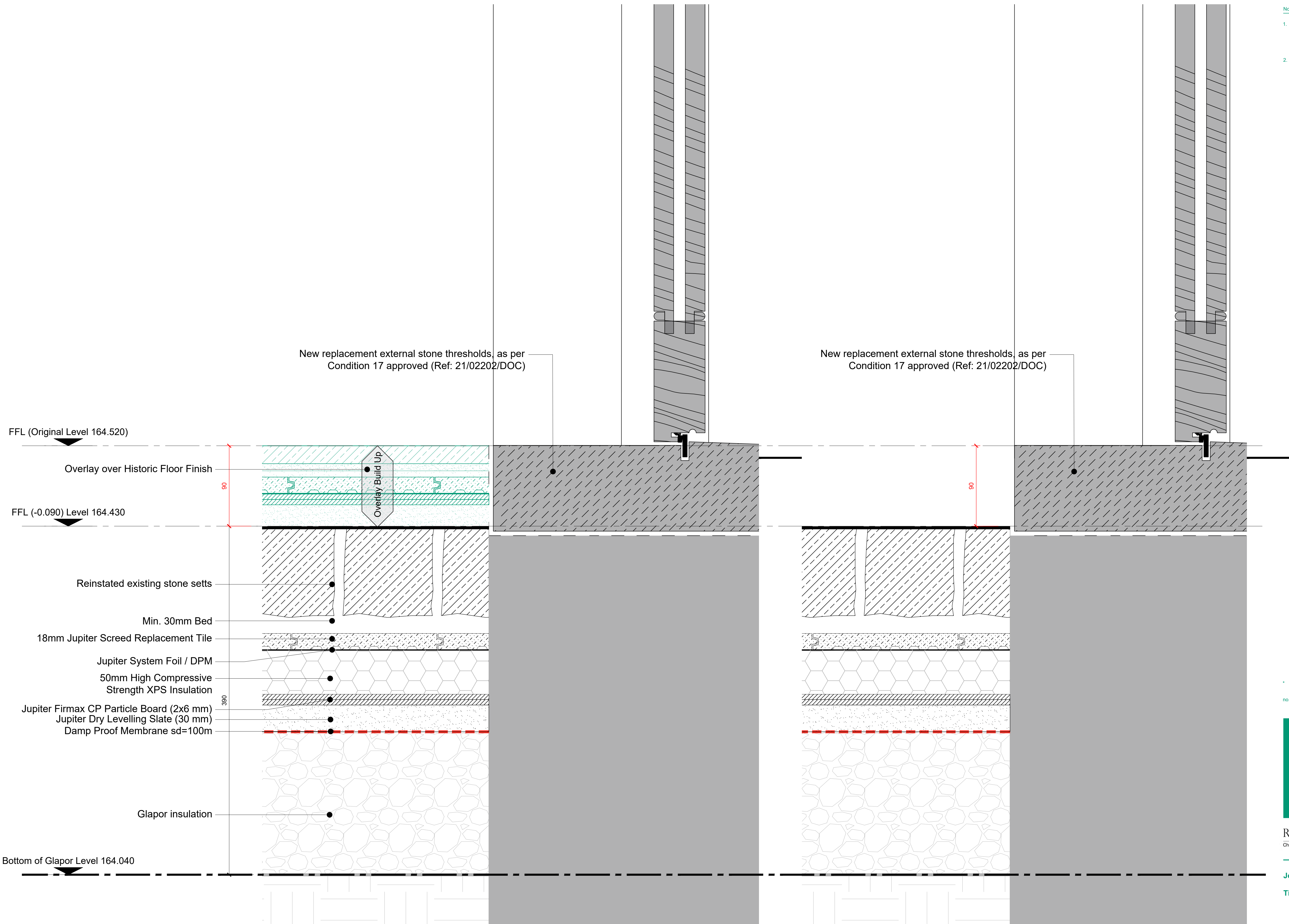
1 Floor Build ups - External Door Threshold Detail with overlay 1:2 @ A1 / 1:4 @ A3 - GROUND FLOOR
