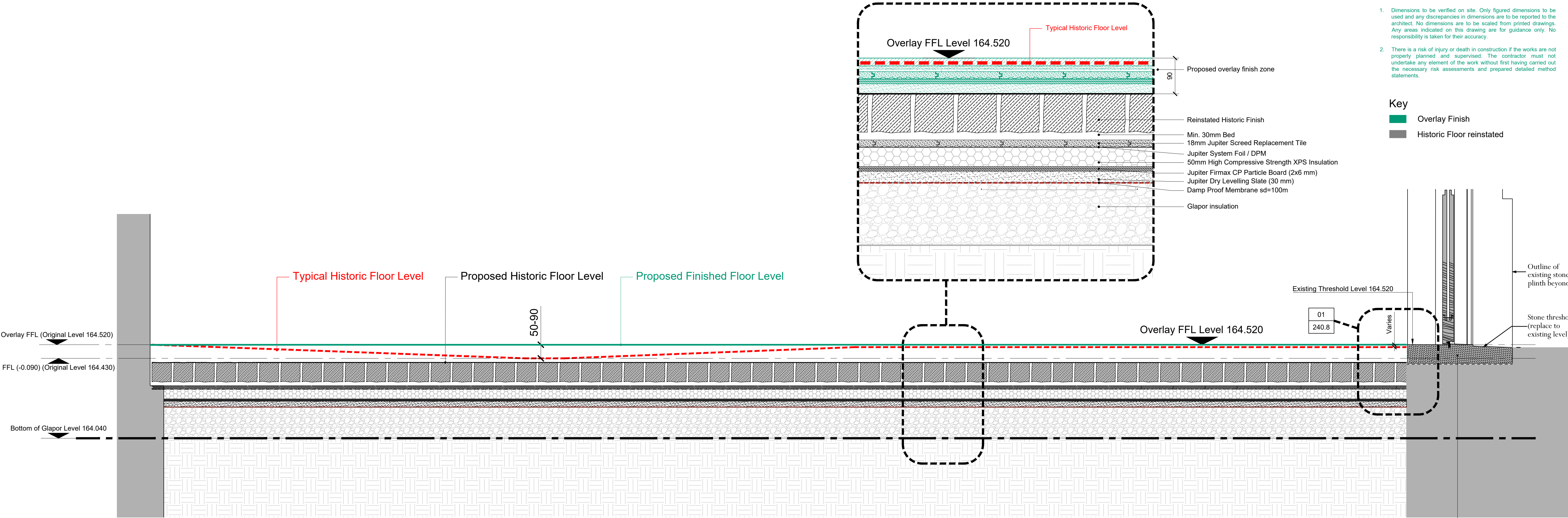
1 Typical Ground Floor Cross Section Build Up / Existing & Proposed 1:10 @ A1 / 1:20 @ A3 - GROUND FLOOR
