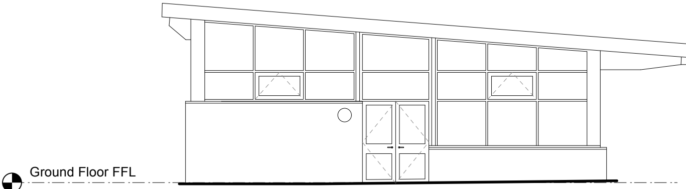
SE Proposed South-East Elevation Scale 1:100
