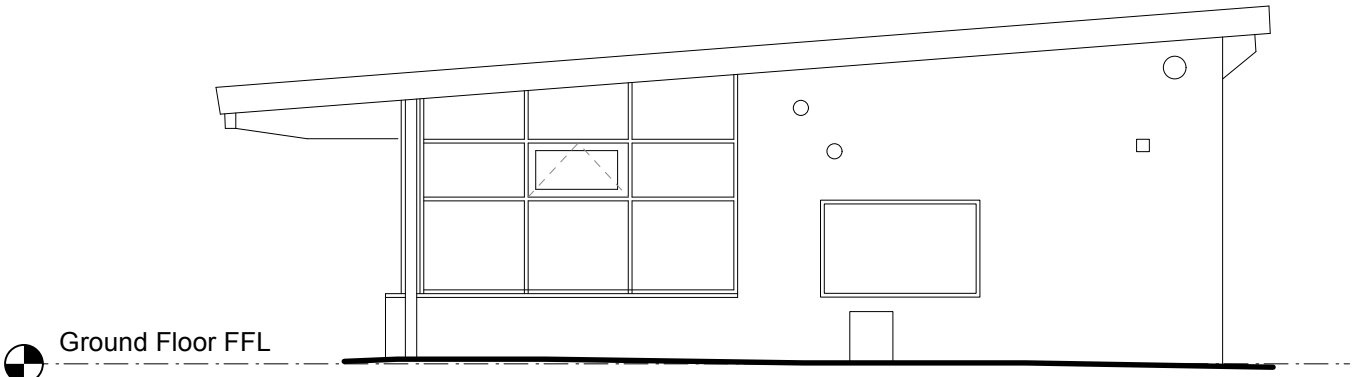
NW Proposed North-West Elevation Scale 1:100
