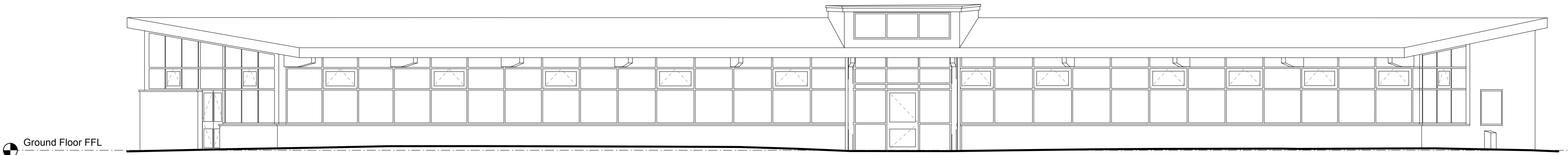
NE Proposed North-East Elevation Scale 1:100
