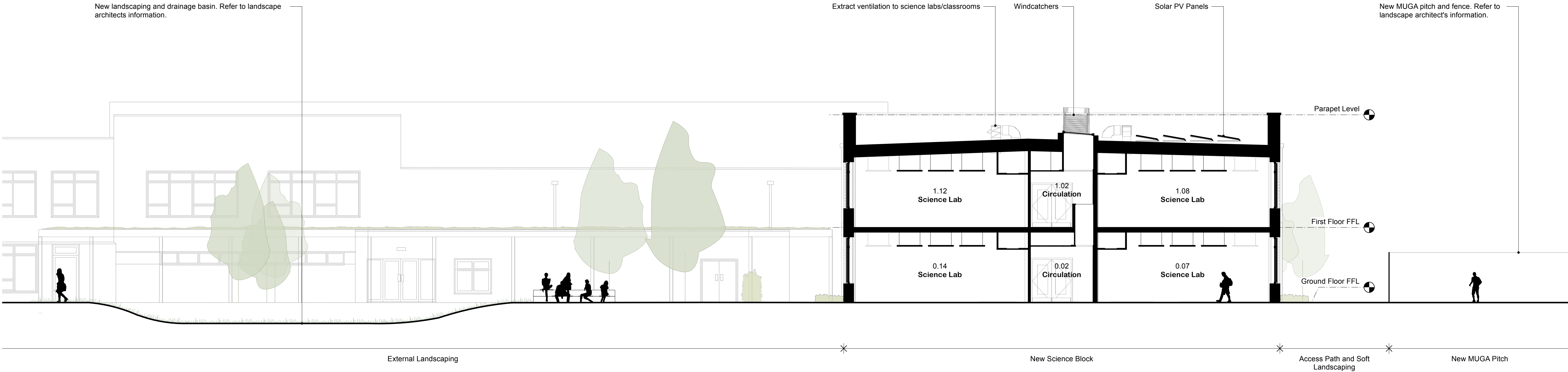
A-A Proposed Section A-A Scale 1:100
