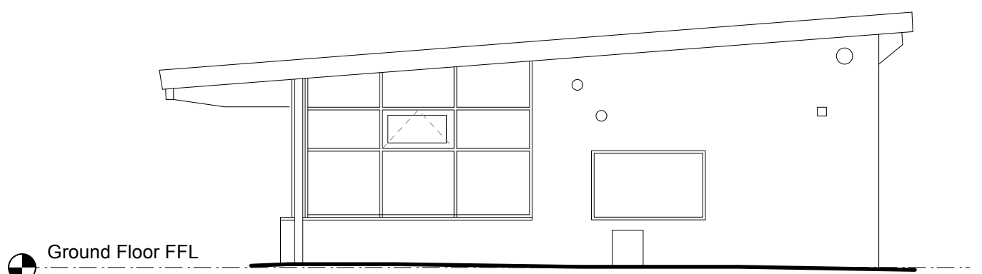
NW Existing North-West Elevation Scale 1:100
