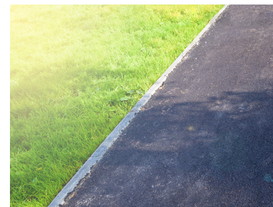
Concrete Edging Description: To macadam path edges and surface changes Colour/Finish: Silver (or acceptable equivalent) To engineer's specification
