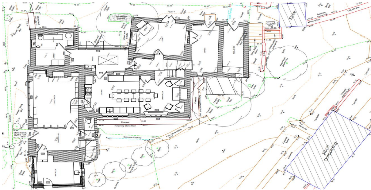
Figure 10 – Existing ground floor layout.
