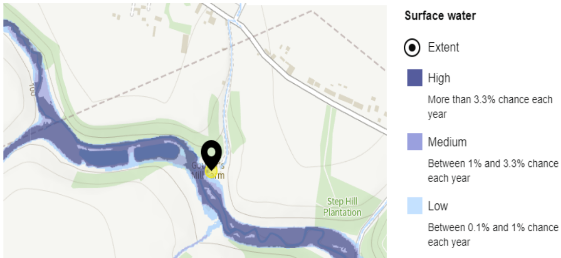
Figure 5 – Flooding from surface water sources, uFMfSW, site highlighted.
