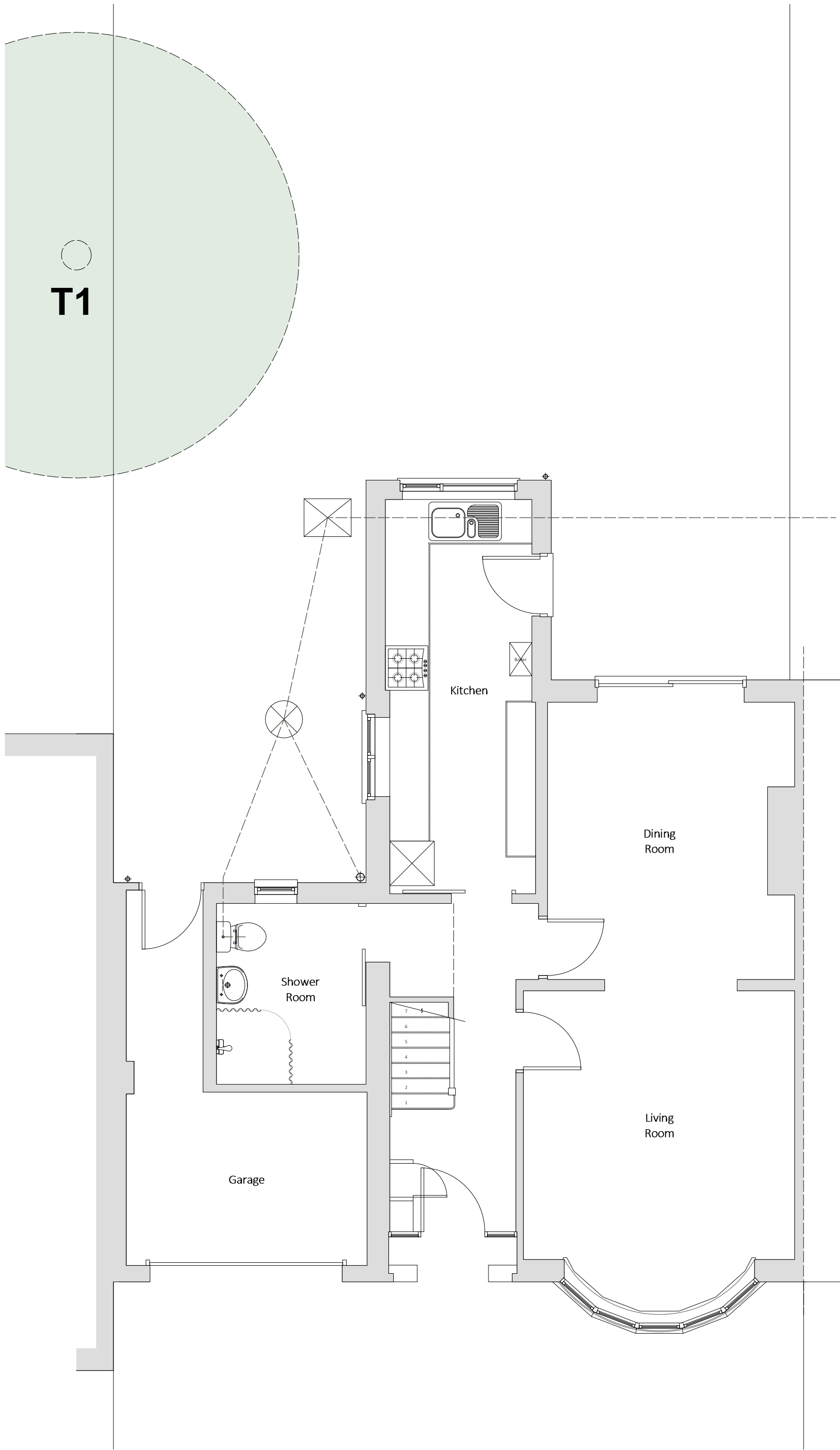
PLN 01 Existing GF Plan 1:50
