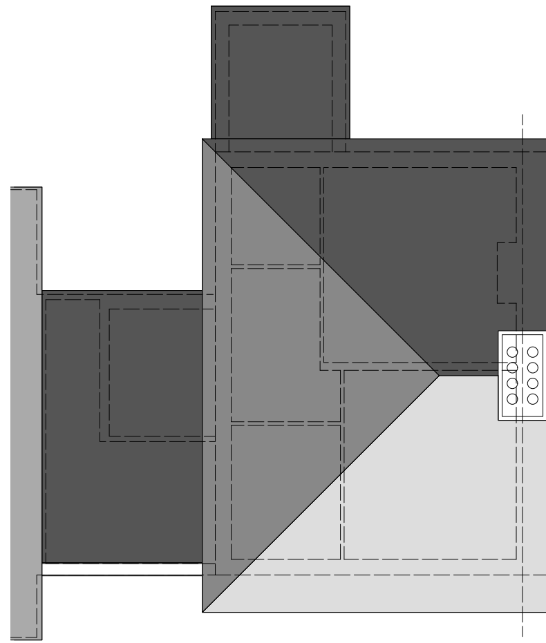
PLN 03 Existing Roof Plan 1:100
