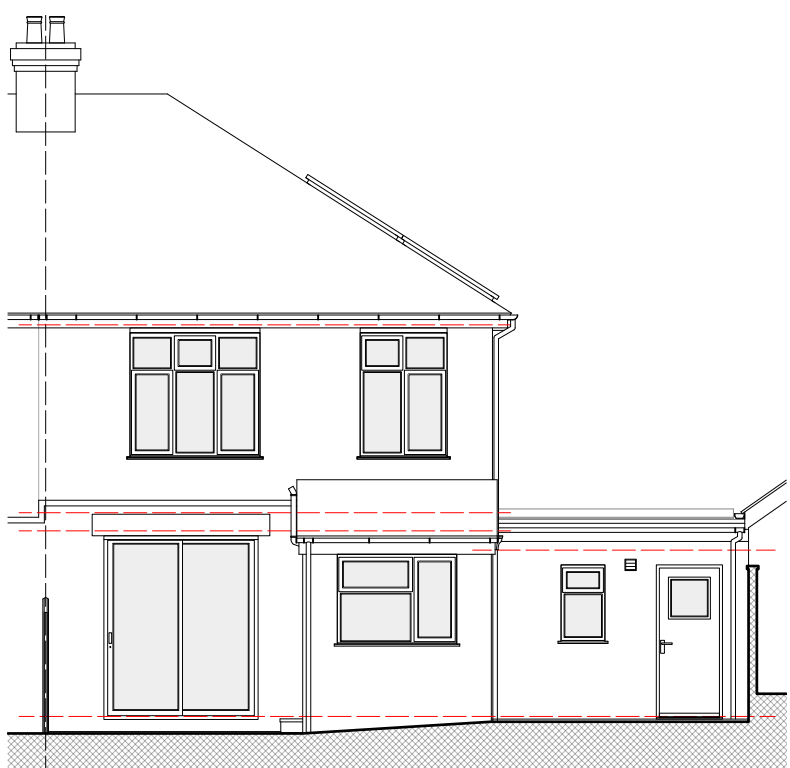
ELV 03 Existing N Elevation 1:100
