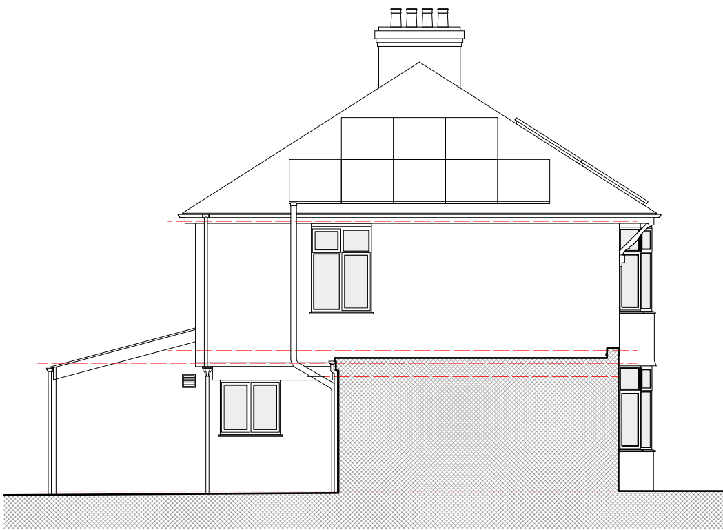
ELV 02 Existing W Elevation 1:100
