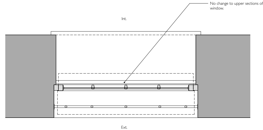
04 - Upper Plan Typical
