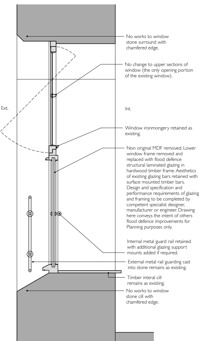
05 - Section - Typical
