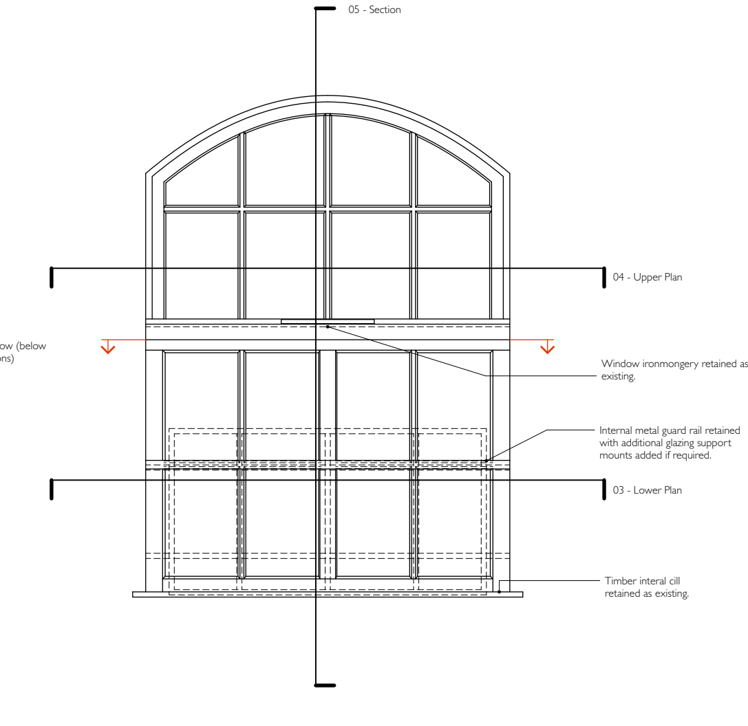
02 - Inside elevation - Typical
