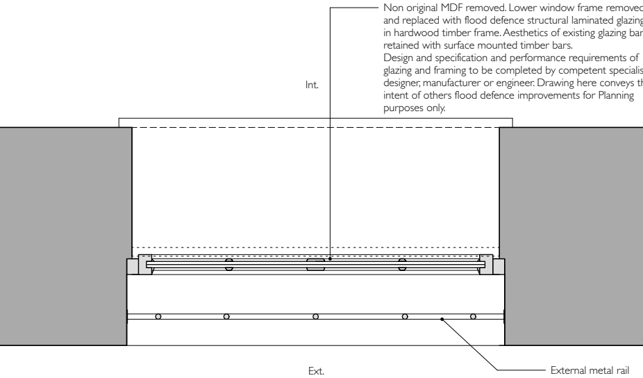
03 - Lower Plan Typical
