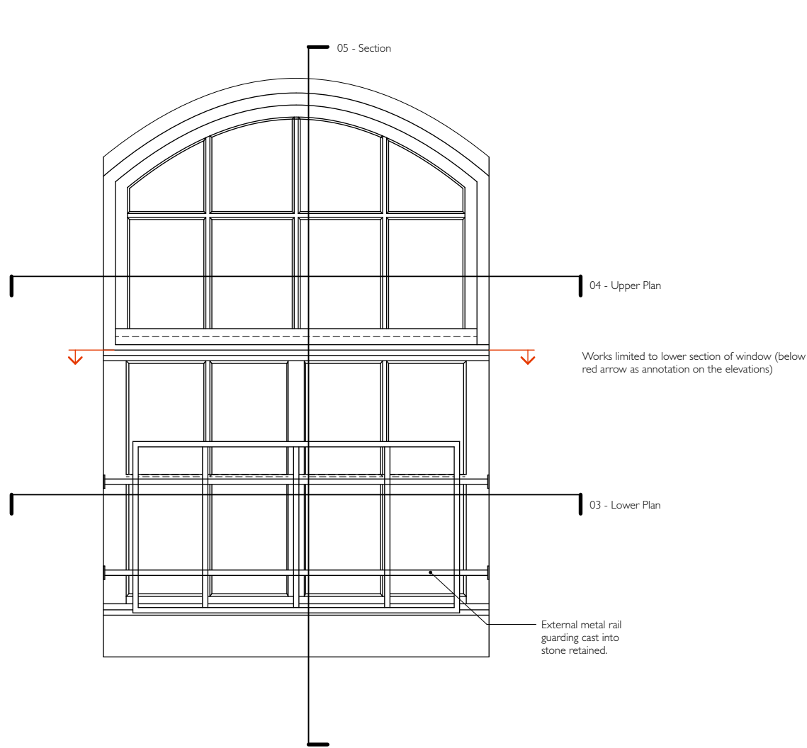
01 - Outside elevation - Typical
