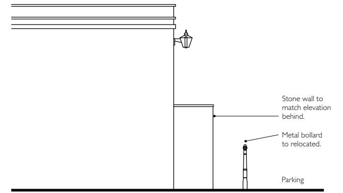
05 - North Elevation - Scale 1:100
