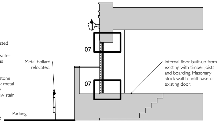
04 - Section - Scale 1:100
