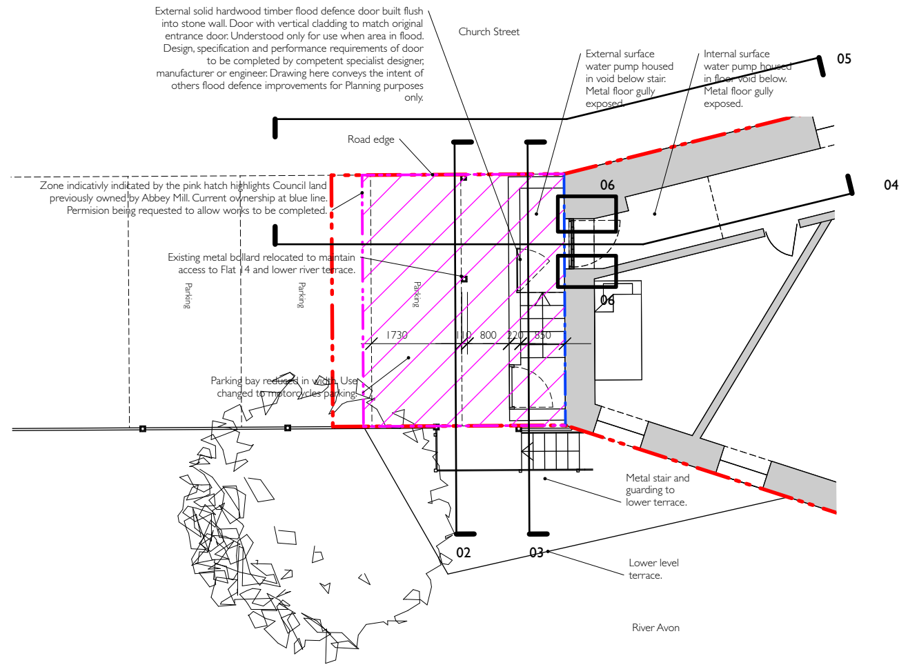
01 - Plan - Scale 1:100
