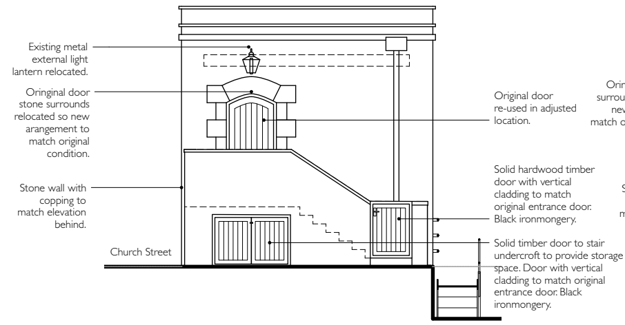
02 - West Elevation - Scale 1:100
