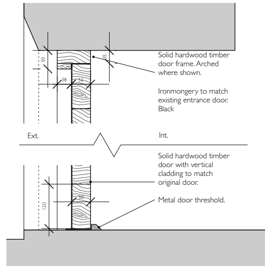
07 - Solid hardwood timber door section - Typical to match existing entrance door- Scale 1:10
