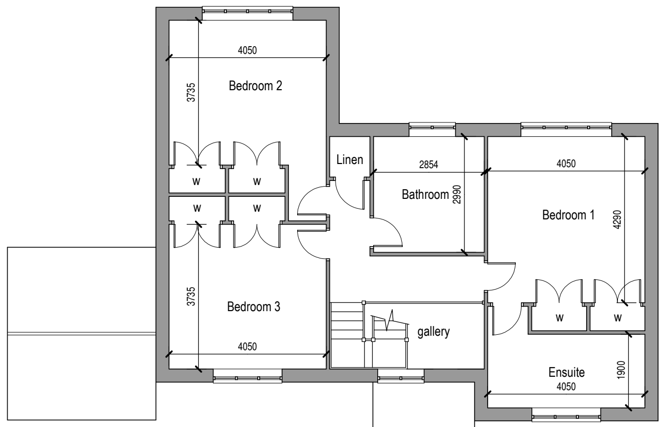
FIRST FLOOR PLAN - 89m²
