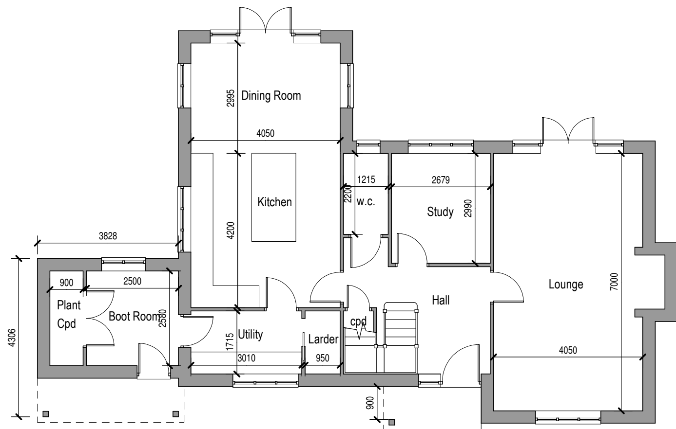
GROUND FLOOR PLAN - 99m²
