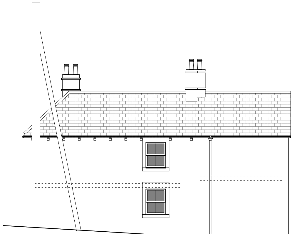
SIDE (E) ELEVATION - scale 1:100
