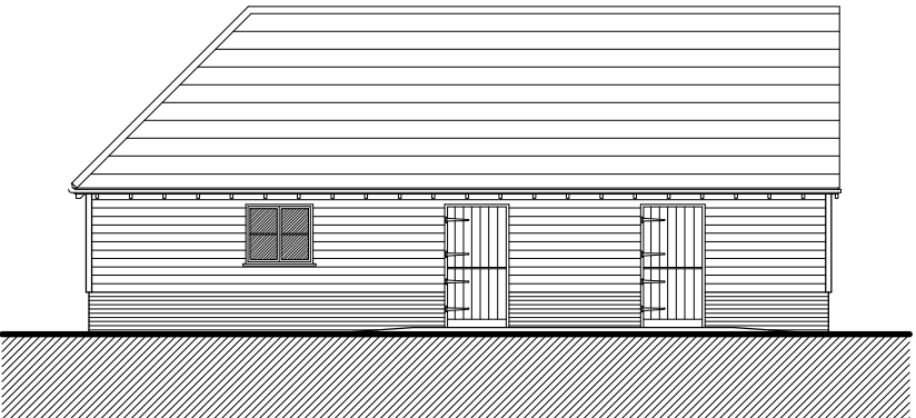
West Elevation
