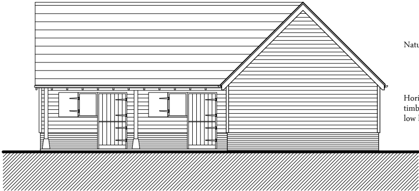
East Elevation
