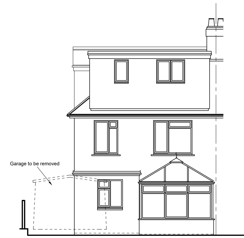
SOUTH (rear)
