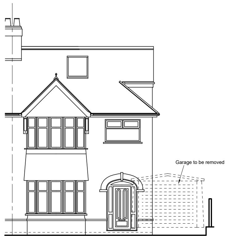
NORTH (front) EXISTING ELEVATIONS scale 1:100
