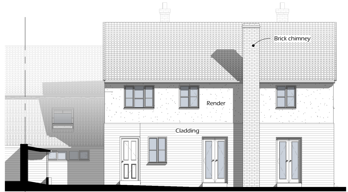
1 North Elevation 1 : 100
