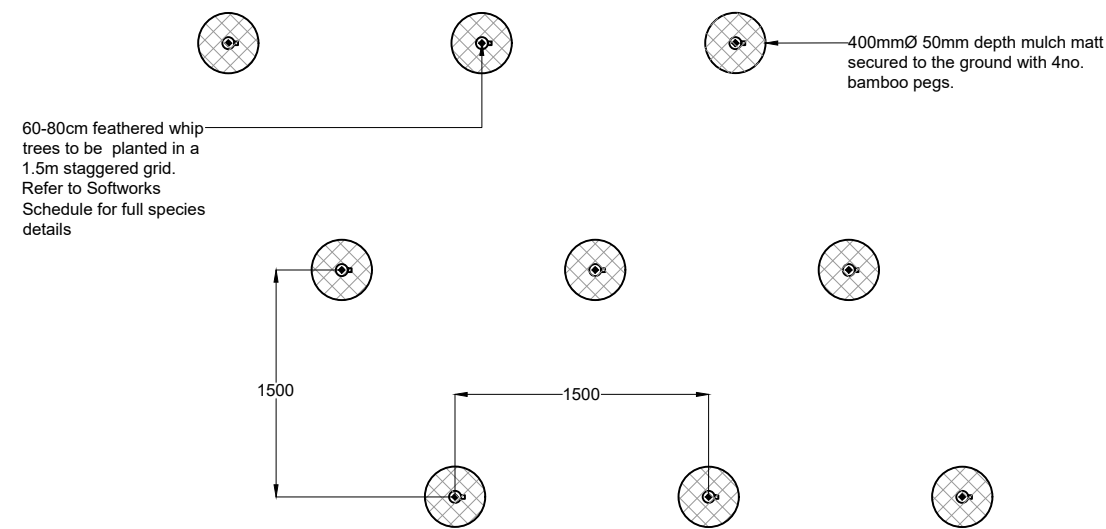
PROPOSED WOODLAND PLANTING PLAN LAYOUT
