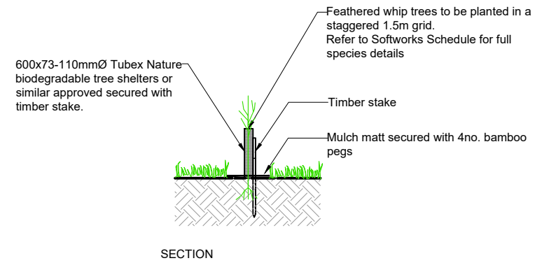
PROPOSED WOODLAND PLANTING
