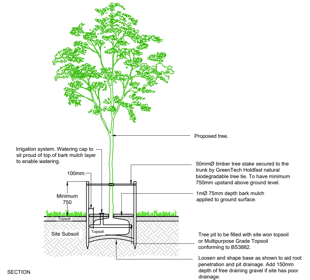
PROPOSED TREE PLANTING TO BE DOUBLE STAKED
