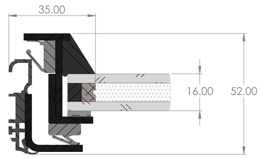
DETAIL A-1 STEELYTE SLIM OPENER SCALE 1:1
