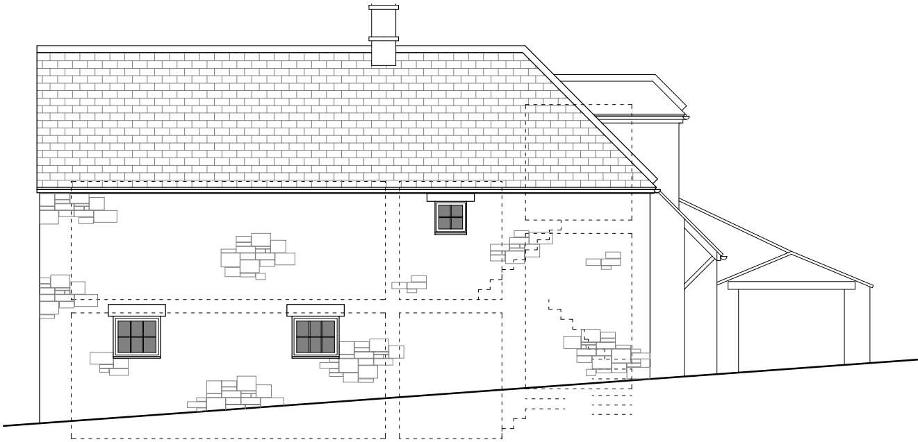
FRONT (NE) ELEVATION - scale 1:100
