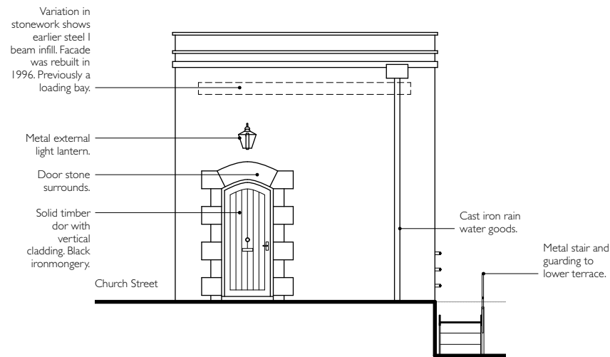
02 - West Elevation
