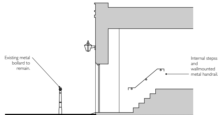
03 - Section
