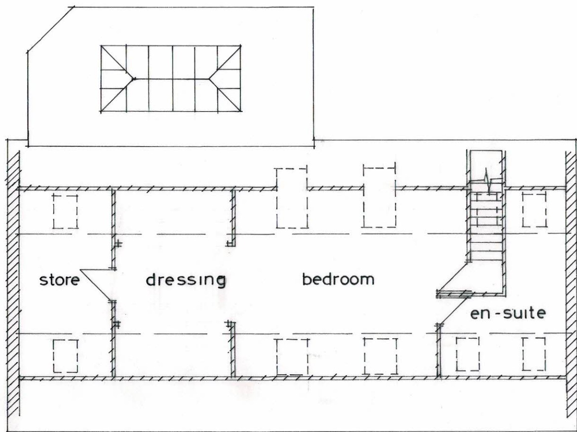
FIRST FLOOR
