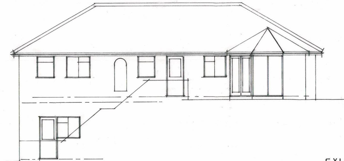
SOUTH WEST
