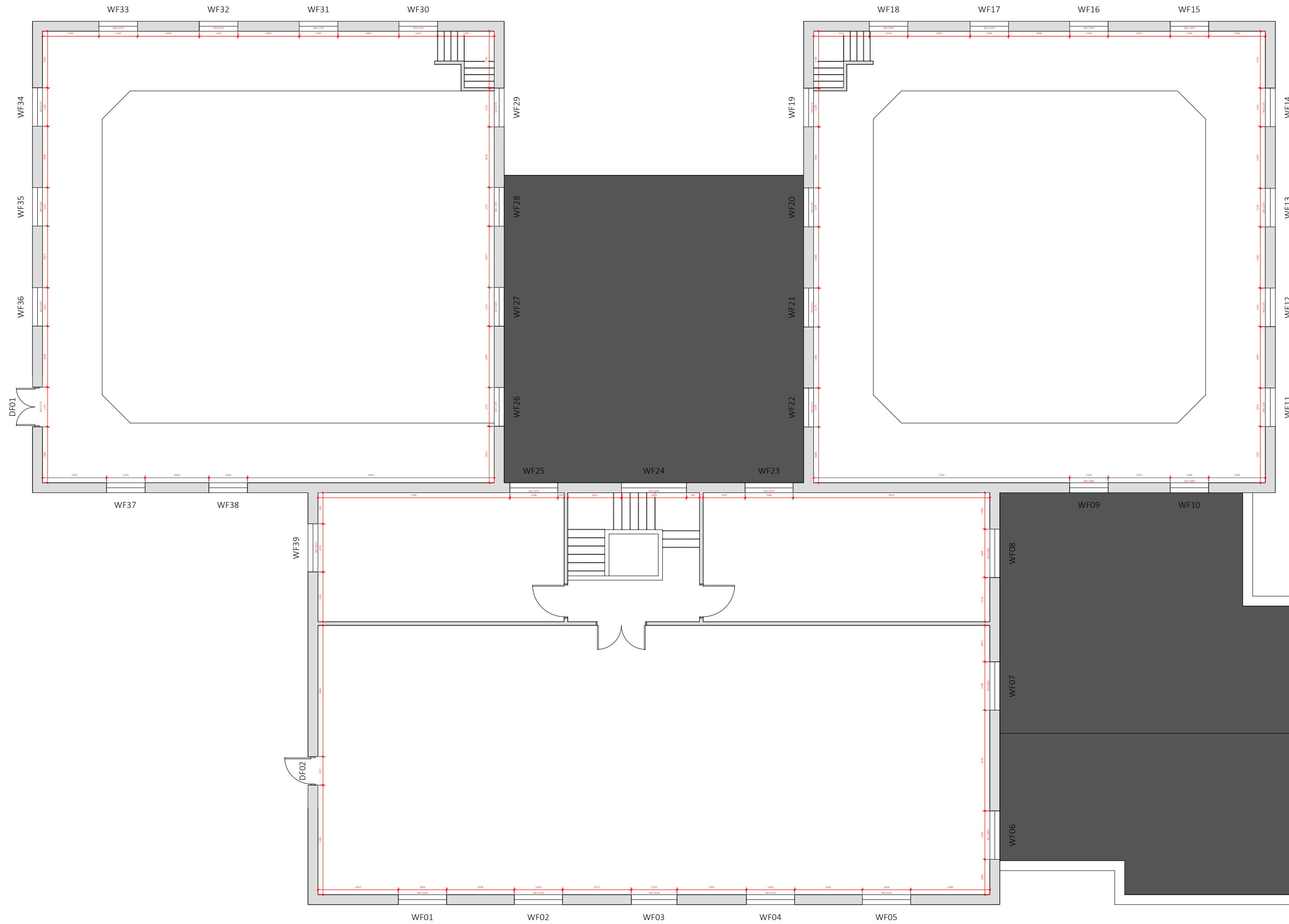
PLN Existing FF Plan 01 1:100
