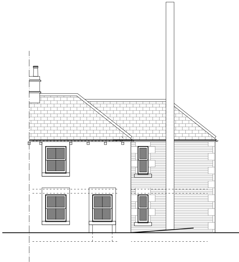
FRONT (S) ELEVATION - scale 1:100
