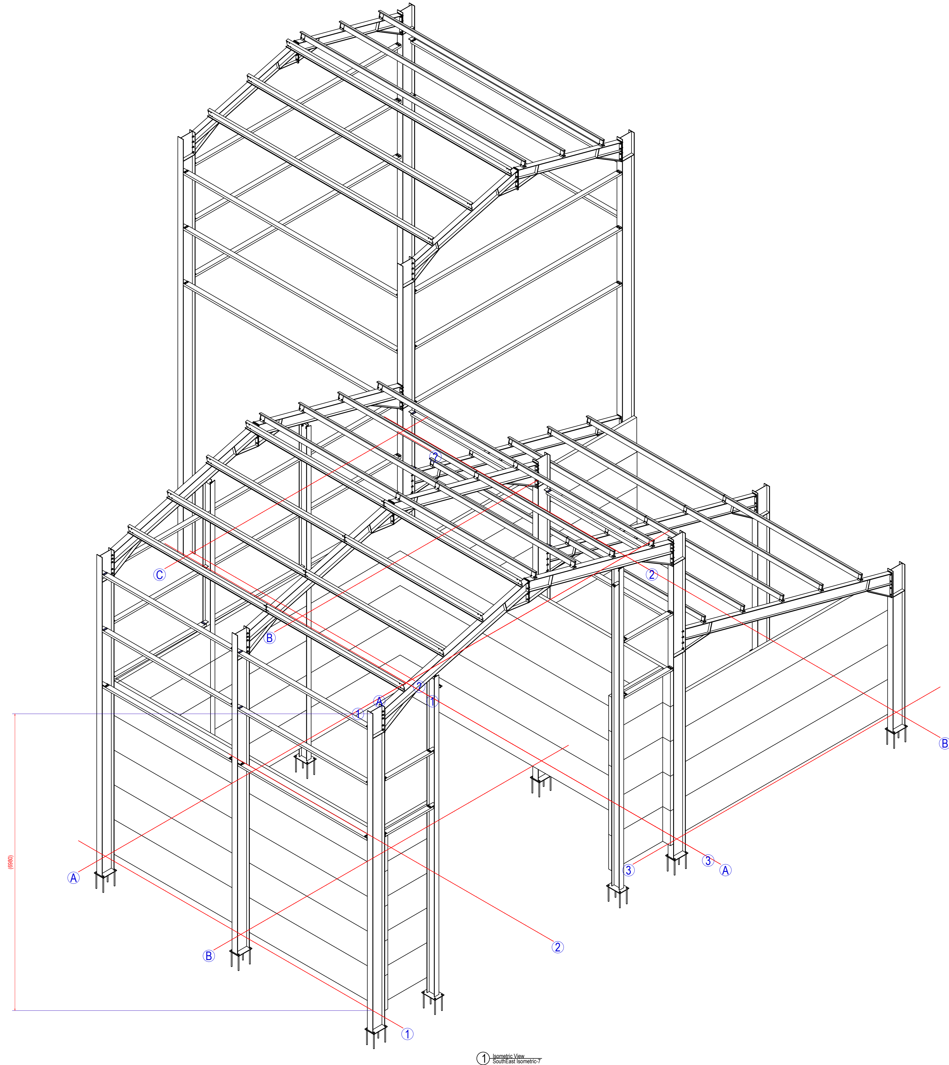
① Isometric View South-East Isometric
