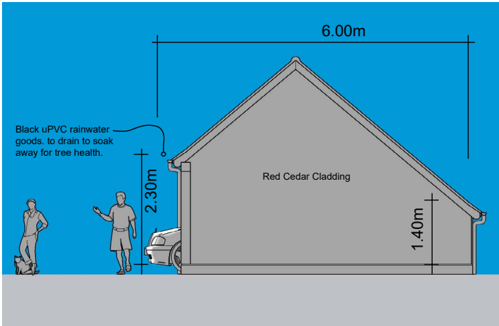
Side Elevation of Garage Port
