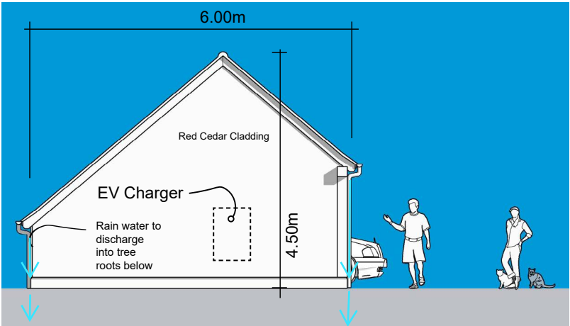
Side Elevation of Garage Port
