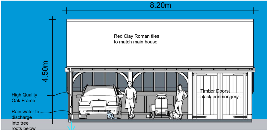
Front Elevation of Garage Port
