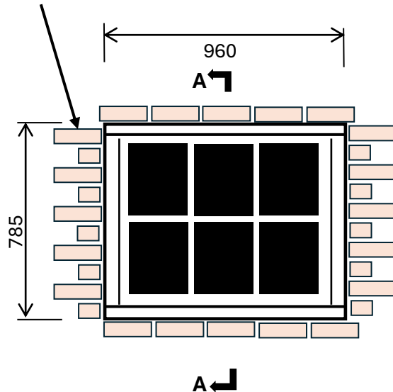
Elevation of Proposed Window (Scale: 1.20 @ A4)
