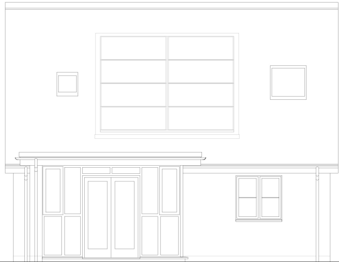
Rear Elevation
