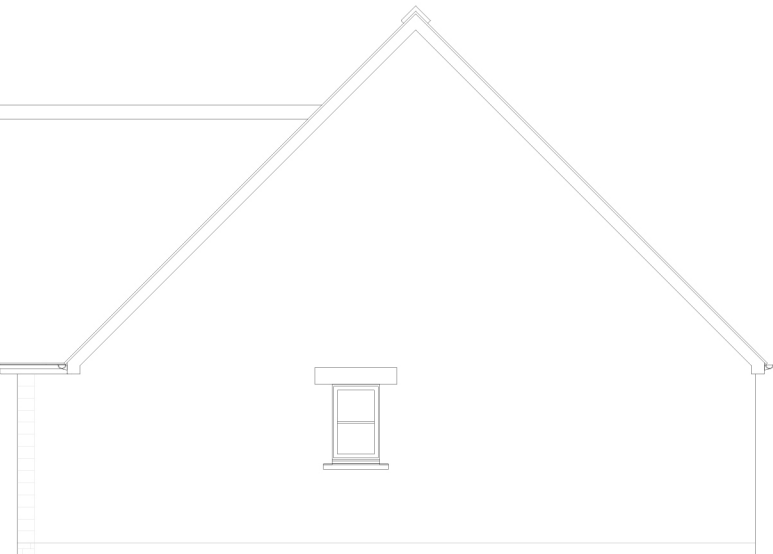
Side Elevation
