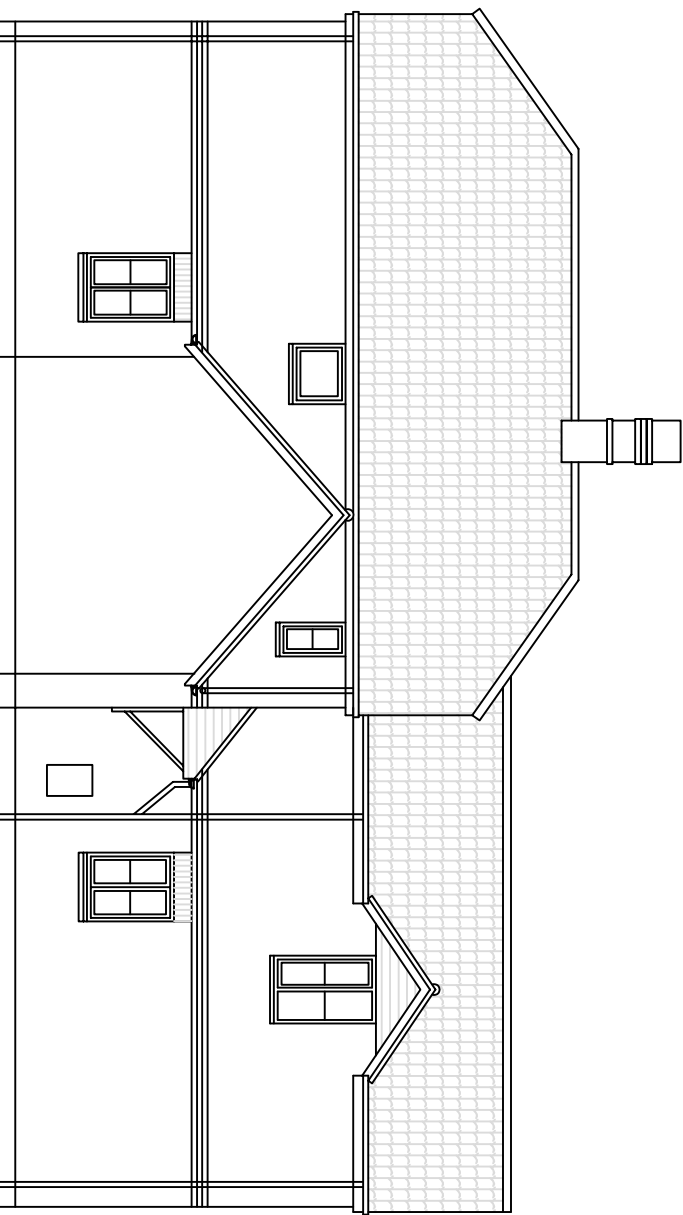
Existing Front (North) Elevation 1:100
