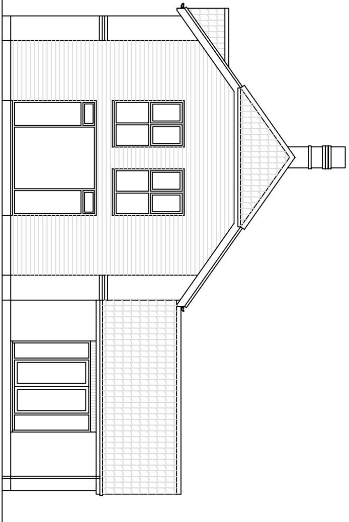
Existing Side (East) Elevation 1:100
