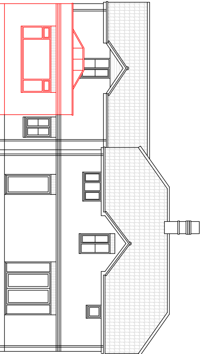
Existing Rear (South) Elevation 1:100
