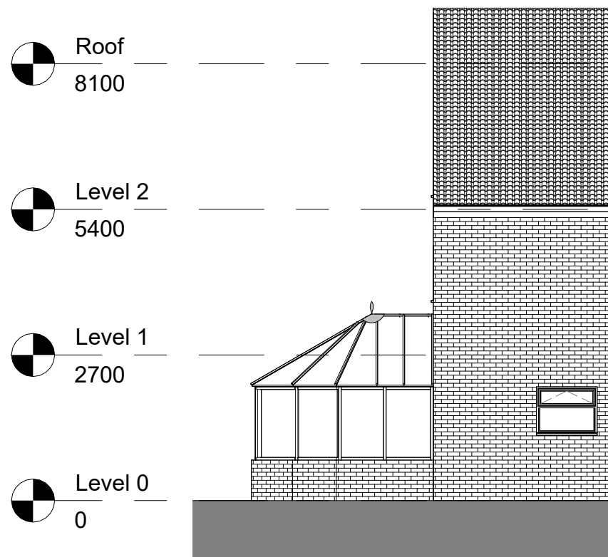
3 North-East Elevation Existing 1 : 100
