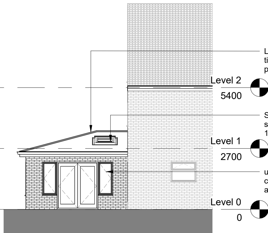
4 North-East Elevation Proposed 1 : 100
