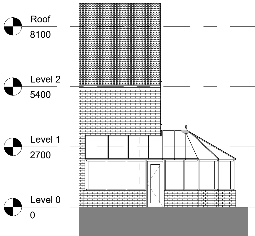
1 South-West Elevation Existing 1 : 100
