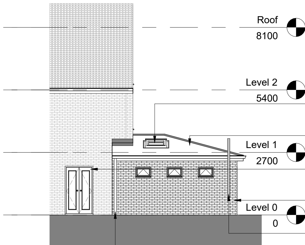
2 South-West Elevation Proposed 1 : 100
