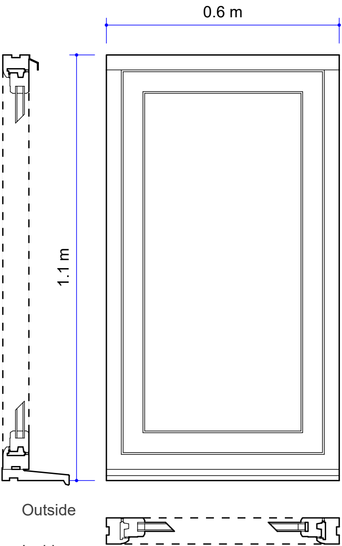
Type 1 - One casement, overall size = 0.71 sqm clear glazing = 0.38 sqm
