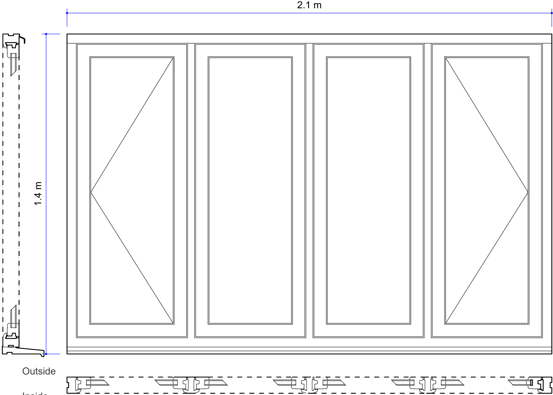
Type 4 - Four casement, overall size = 2.94 sqm / clear glazing = 1.76 sqm
